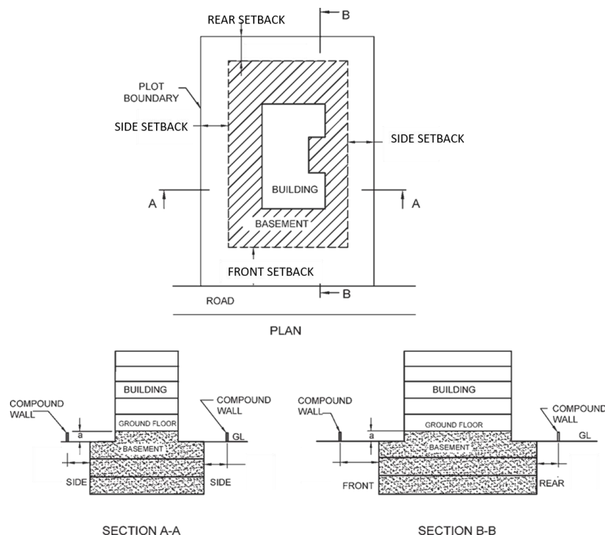
Figure 24 Basement
